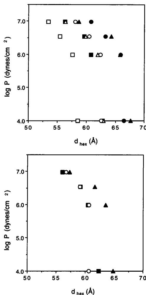
FIGURE 3 Plots of the relation between lattice dimension of the hexagonal phases and the osmotic pressure of the PEG solution with which they are equilibrated. Data are shown for a variety of temperatures, as indicated for the three lipids \Delta 6 PE ( \square , \blacksquare ), \Delta 9 PE ( \circ , \bullet ), and \Delta 11 PE ( \triangle , \blacktriangle ). (Upper panel) T_H ( \bullet , \blacksquare , \blacktriangle ) and T_H + 20^\circ ( \circ , \square , \triangle ). (Lower panel) T = 40^\circ\text{C} .
