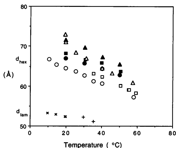
FIGURE 2 The temperature dependence of the hexagonal ( \circ , \bullet , \square , \blacksquare , \triangle , \blacktriangle ) and lamellar ( + , \times ) lattice spacings, both with ( \bullet , \blacksquare , \blacktriangle ) and without ( \circ , \square , \triangle ) 16 wt% added tetradecane, for the three lipids in excess water. \square , \blacksquare , + , \Delta 6 PE; \circ , \bullet , \Delta 9 PE; \triangle , \blacktriangle , \times , \Delta 11 PE. Without tetradecane, the lowest experimental temperature at which a single hexagonal phase exists coincides closely with T_H for each lipid, as measured by DSC (Table 1).
